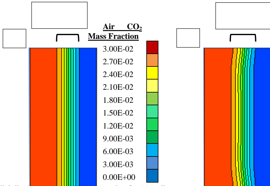
Fig. 14: Radial distributions of CO 2 concentration for (a) wall temperature of 20°C and (b) wall temperature of -1°C
